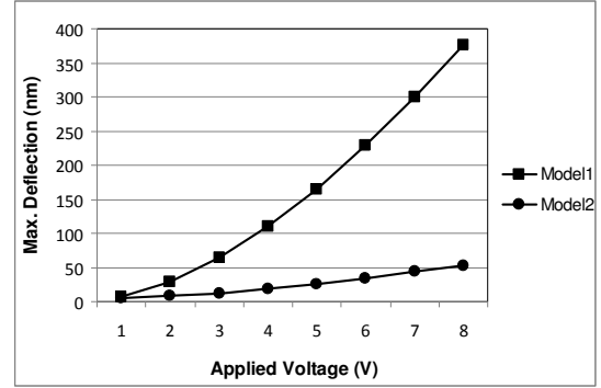
Fig.5. Comparison of deflections in Model-II using Poly-Si with Model-I using the same material
