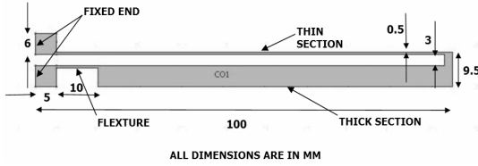
Fig.1. Basic geometry of Model-I & III
