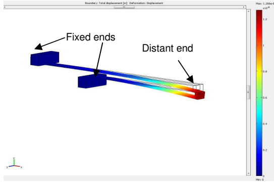
Fig.4. Deflection of Model-II
