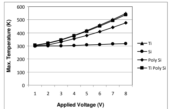
Fig.7. Comparison of temperatures for Model-III (Ti-Poly Si) with Model-I (Ti, Si, Poly-Si)
