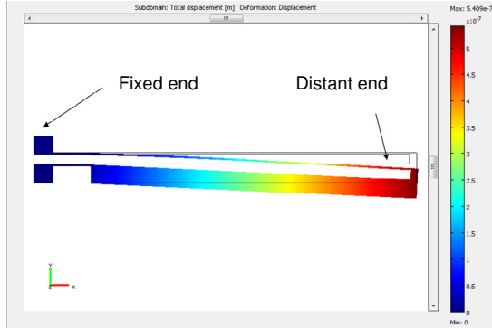
Fig.3. Deflection of the actuator
