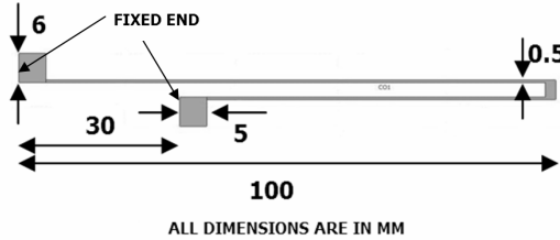
Fig.2. Basic geometry of Model-II
